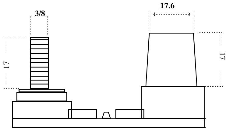
Positive Terminal
