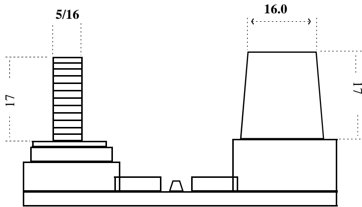
Negative Terminal
